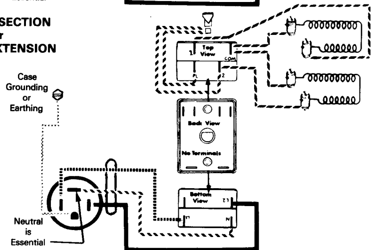
BOTTOM SECTION
