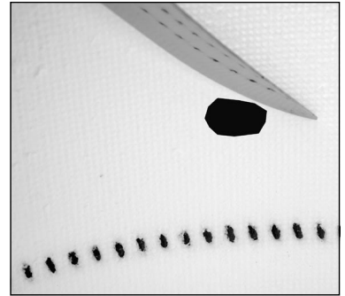
Removing spattered glaze from the ceramic fiber wall with a knife. Caution: unplug kiln. Avoid disturbing the element.
