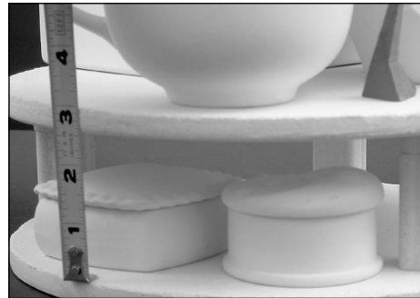
Posts in each layer should be at least 1" taller than the ware. Minimum spacing between shelves is 2 1/2" as shown above.
